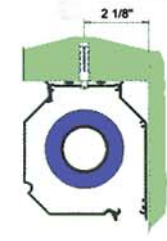
Ceiling mount through top of box
