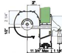
Through wall crank operation • small gear
