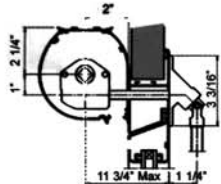
Through wall crank operation • large gear
